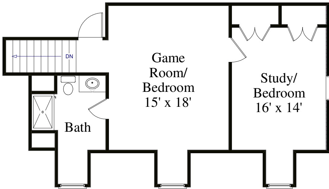
Third Floor
